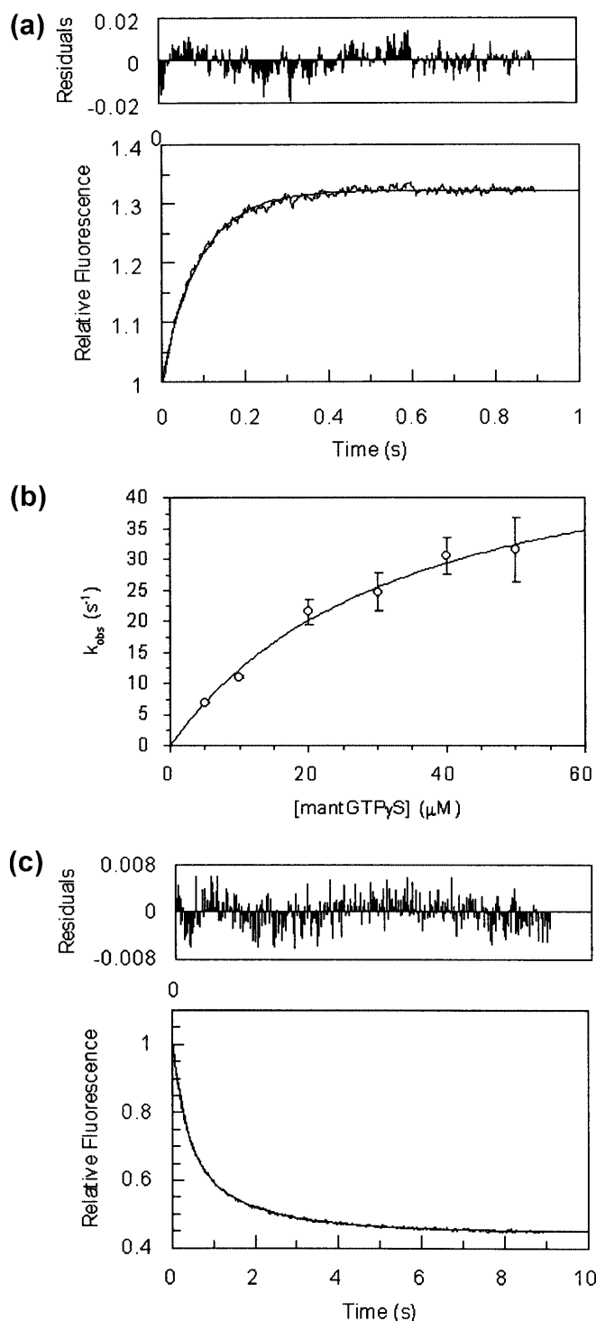
Fig. 2a–c. Interaction of mantGTP \gamma S with dynamin II. (a) Stopped-flow fluorescence record of the binding of mantGTP \gamma S to dynamin II. 1 \mu\text{M} dynamin II was rapidly mixed with 10 \mu\text{M} mantGTP \gamma S at 20 °C. The solid line is the best fit of the data to a single exponential with a rate constant of 10.8 \text{ s}^{-1} . (b) Dependence of the rate constant on the concentration of mantGTP \gamma S. Data were obtained from experiments as in (a). The solid line is the best fit to a two-step binding model described by Binns et al. (2000). (c) Stopped-flow fluorescence record of the displacement of mantGTP \gamma S from dynamin II. 1 \mu\text{M} dynamin II and 2 \mu\text{M} mantGTP \gamma S was rapidly mixed with 100 \mu\text{M} GTP at 20 °C. The solid line is the best fit to a single exponential with rate constants of 2.77 \text{ s}^{-1} (amplitude 63%) and 0.56 \text{ s}^{-1} (amplitude 37%)
