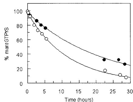
Fig. 1. Hydrolysis of mantGTP \gamma S by dynamin II. A solution of 1 \mu\text{M} mantGTP \gamma S and 10 \mu\text{M} dynamin II in 20 mM HEPES (pH 7.4), 300 mM NaCl, 5 mM \text{MgCl}_2 , 1 mM EDTA and 0.5 mM dithiothreitol was incubated at 20 °C (filled circles) or 30 °C (open circles). Samples were analysed for mantGTP \gamma S and mantGDP by HPLC. The lines are the best fits of the data to single exponentials with rate constants of 1.33 \times 10^{-5} \text{ s}^{-1} at 20 °C and 2.33 \times 10^{-5} \text{ s}^{-1} at 30 °C
