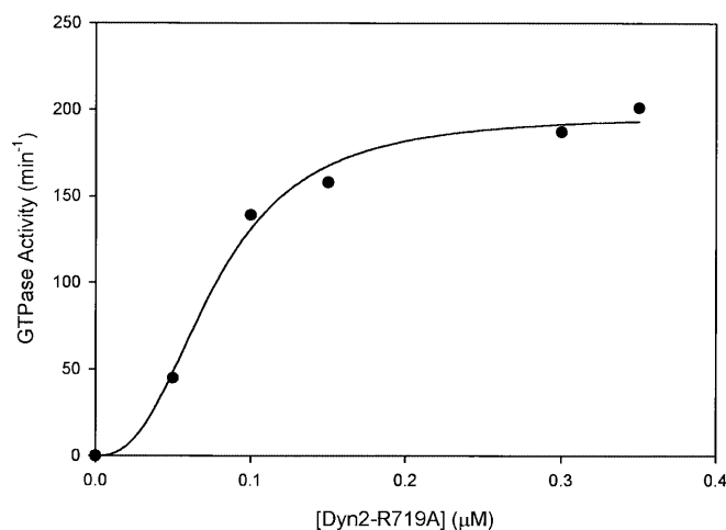
Fig. 3. Activation of dynamin II R719A. The steady-state GTPase activity was measured over the range of concentrations of dynamin II R719A shown. The solution also contained 20 mM HEPES (pH 7.4), 25 mM NaCl, 5 mM \text{MgCl}_2 , 1 mM EDTA, 0.5 mM dithiothreitol, 1 mM GTP and microtubules stabilized with taxol (10 \mu\text{M} tubulin monomer)
